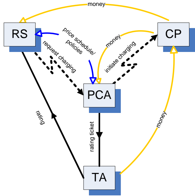
Figure 3. A reputation system with PCA.
